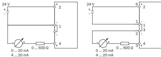
3-wire technology
