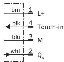
Figure 7: Male connector, M12, 4-pin
