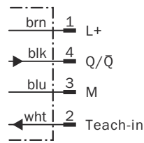
Figure 6: Male connector, M12, 4-pin
