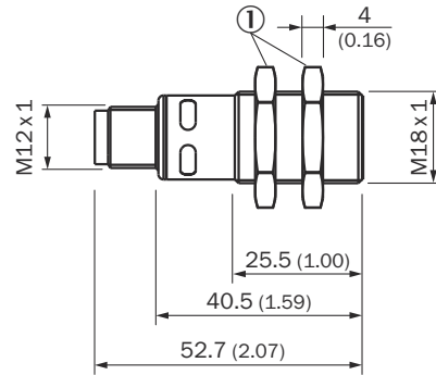
Figure 11: Structure and device dimensions, unit: mm (inch), decimal separator: period
