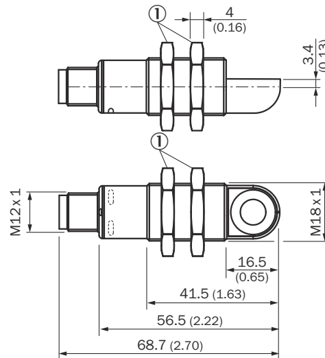
Figure 12: Structure and device dimensions, unit: mm (inch), decimal separator: period
