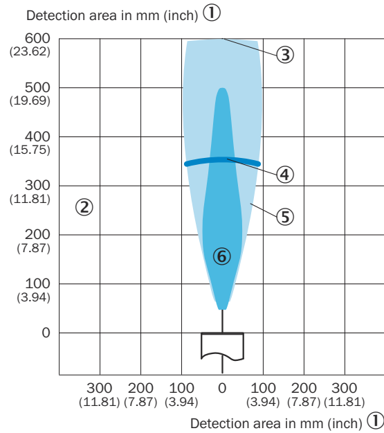
Figure 14: Um18-212xxxxx detection range
