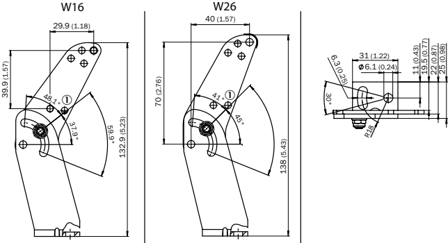
① 0° position
