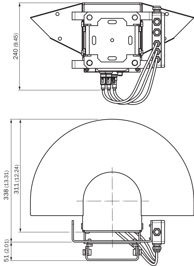
Weather hood, 190°
