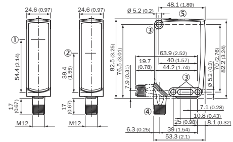
Figure 16: Dimensional drawing 2, male connector
