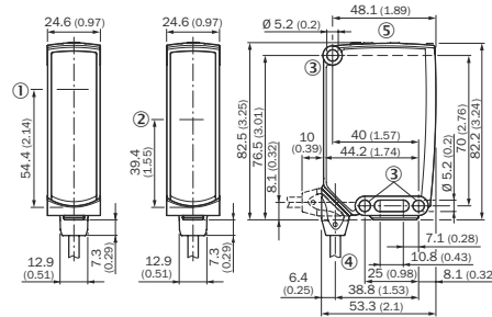
Figure 15: Dimensional drawing 1, cable
