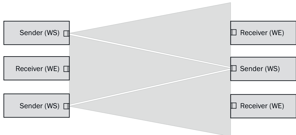
Figure 9: Arrangement of multiple through-beam photoelectric sensors
