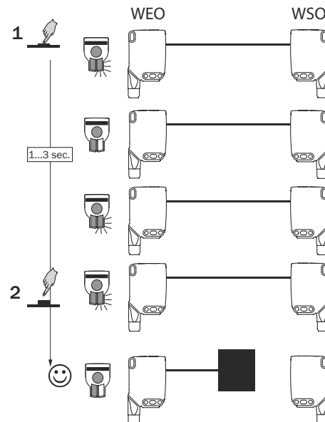
Figure 14: WSE26x-xxxxxx3xAxx, adjusting the sensing range with teach-in button
