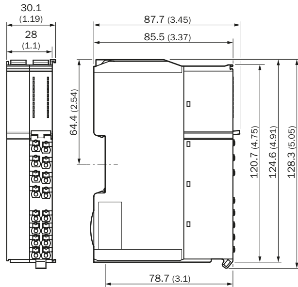
RLY3-OSSD400 relay module
