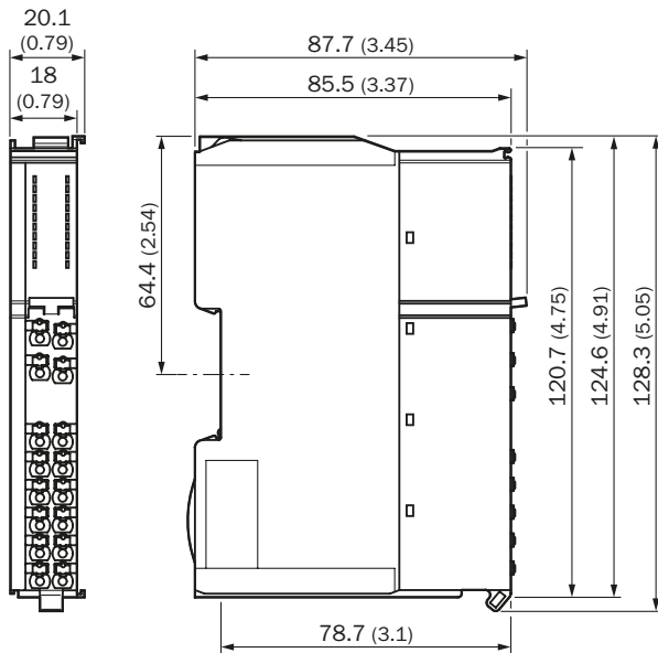
RLY3-OSSD100 relay module
